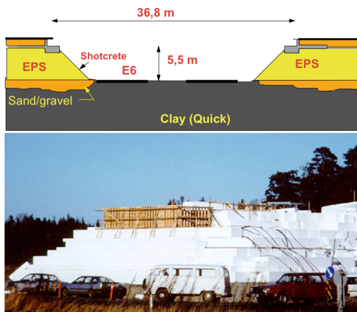
Figure 1. Abutment on EPS at Løkkeberget bridge
